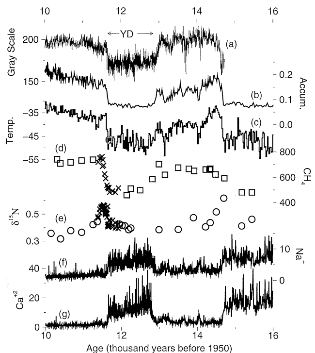
Fig. 1. High-resolution data from the GISP2 ice core and from the Cariaco Basin, covering the abrupt onset of the Bolling/Allerod warm period, the cool Younger Dryas interval (YD), and the warming into and through the Preboreal that followed. (a) Gray-scale data from Hughen et al. (1996, 1998) for a core from the Cariaco Basin, offshore Venezuela. The gray scale is affected by productivity in response to wind-driven upwelling, with lower numbers corresponding to enhanced windiness. Note that the time scale for this record was derived independently of those for the ice core. (b)–(e) Data mostly from Severinghaus et al. (1998), with the accumulation and temperature originally from Cuffey and Clow (1997). (b) Accumulation in to m ice/yr. (c) Temperature converted from ice-isotopic ratios (Grootes & Stuiver, 1997) using the glacial-interglacial calibration of Cuffey et al. (1995), shown in degrees C. The Severinghaus et al. (1998) estimate of temperature in the Younger Dryas is plotted as a circle; uncertainties of about \pm 3^\circ\text{C} are not much larger than the symbol. (d) Methane data (ppbv) from Brook, Sowers and Orcharo (1996) (squares) and Severinghaus et al. (1998) (x). (e) \delta^{15}\text{N} data in per mil are from Severinghaus et al. (1998), with (o) from their Fig. 2 and (x) from their Fig. 4. (f)–(g) Sodium (f) and calcium (g) data from Mayewski et al. (1997), normalized to their mean concentration in the millennium before the Little Ice Age following Alley et al. (1997) using the accumulation-rate estimates of Alley et al. (1993). Most of the ice-core data, and many related data sets, are available on The Greenland Summit Ice Cores CD-ROM, 1997, National Snow and Ice Data Center, University of Colorado at Boulder, and the World Data Center-A for Paleoclimatology, National Geophysical Data Center, Boulder, Colorado, www.ngdc.noaa.gov/paleo/icecore/greenland/summit/index.html .
